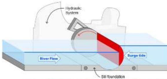
Rising Sector Gate Closed Position
